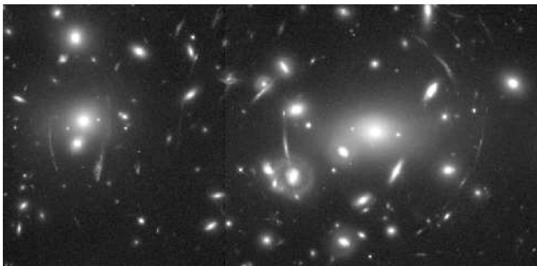
Fig. 8.26 Partial Einstein rings from several sources at varying distances produced by the galaxy Abell 2218. The image was made with Hubble Space Telescope; courtesy Professor R.Ellis (California Institute of Technology), Professor W. Crouch (University of New South Wales) and the NASA Space Telescope.
