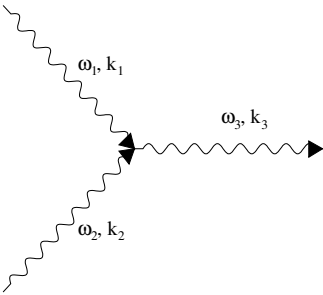
Fig. 14.44 Photon energy-momentum balance in a convertor crystal.
