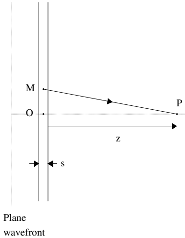
Fig. 11.2 Coherent scattering from a thin plane layer of dielectric.
