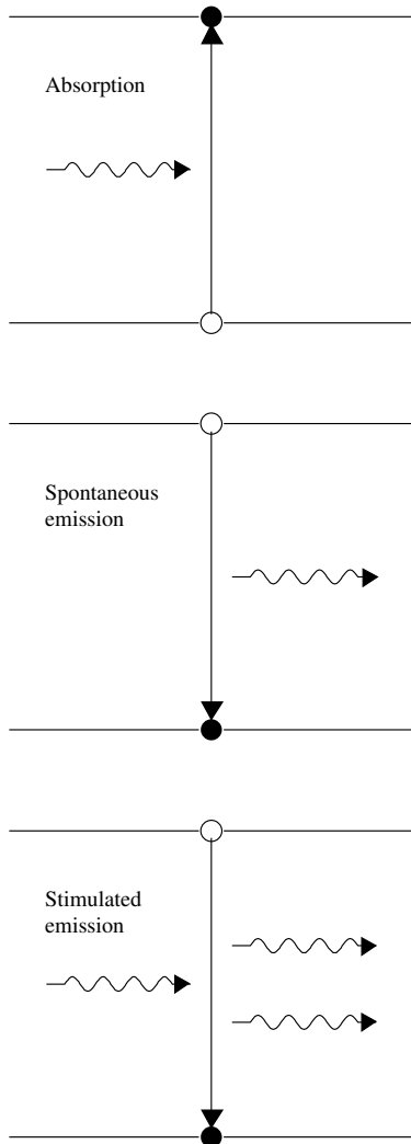
Fig. 14.1 The three photon-matter interactions: in the upper panel absorption; in the centre panel spontaneous emission; and in the lower panel stimulated emission.
