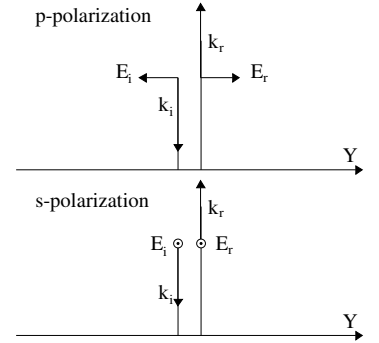
Fig. 9.13 Electric vectors in the incident and reflected waves at normal incidence. Upper panel for p-polarization and lower panel for s-polarization.
