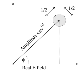
Fig. 18.3 Argand diagram showing the uncertainty in the electric field amplitude for a coherent state.
