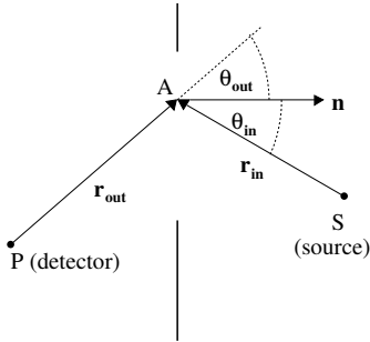
Fig. C.1 The point source S illuminates an aperture. P is the point of observation and A is a representative point on the aperture.
