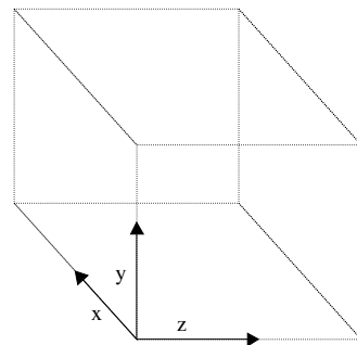
Fig. 9.20 Cubical box used for counting modes.
