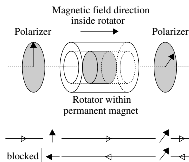
Fig. 10.20 Optical isolator consisting of a Faraday rotator sandwiched between polarizers with their transmission direction inclined at 45^\circ . The polarization states for light travelling in either direction are shown below the device as seen from the left. The Faraday rotator is taken to have a positive Verdet constant.
