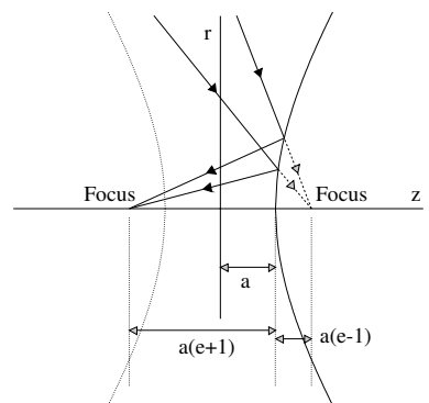
Fig. 8.2 Hyperboloid mirror. The dotted curve shows where the other half of the hyperboloid surface would lie.
