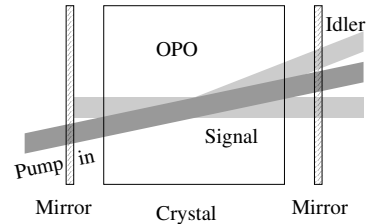
Fig. 14.46 Outline diagrams for the function of an optical parametric amplifier and an optical parametric oscillator.
