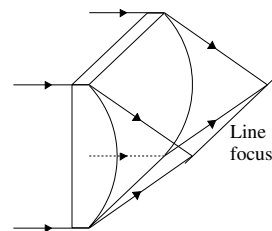
Fig. 3.27 Cylindrical lens.
