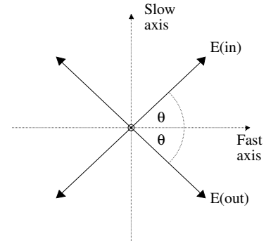
Fig. 10.11 A half-wave plate looking toward the oncoming light. The polarization state of a plane wave is shown before and after passing through the HWP.
