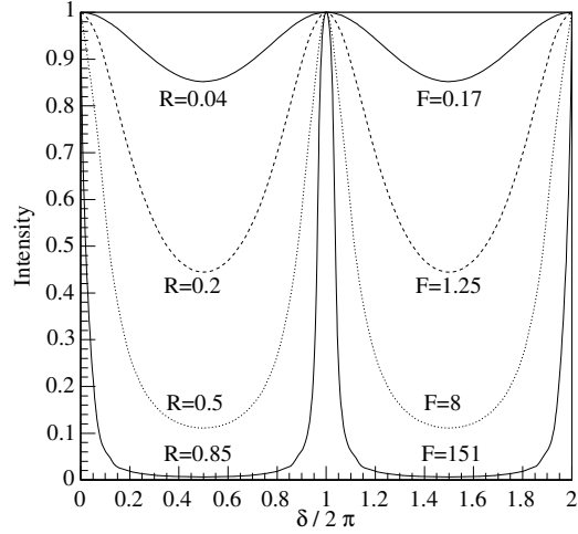
Fig. 5.31 Intensity distribution against \delta/2\pi = 2d \cos \theta / \lambda . The intensity is normalized to the incident intensity.
