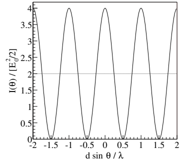
Fig. 5.6 Intensity in Young's two slit experiment as a function of the direction off axis \theta , expressed as a multiple of the single slit intensity. The dotted line shows the mean intensity. \lambda is the wavelength and d the slit separation.
