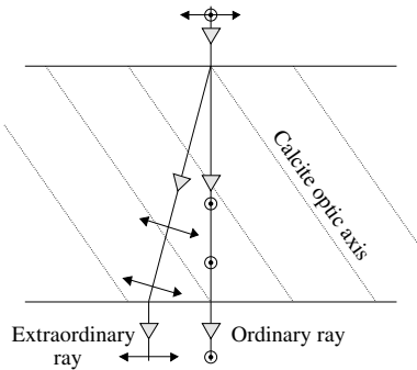
Fig. 10.4 Separation of ordinary and extraordinary rays in passing through a sheet of calcite.
