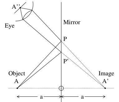
Fig. 2.7 Virtual image A' of point A, distance a from mirror, and focused on the retina at A''.
