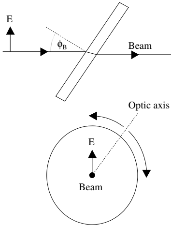
Fig. 14.35 Birefringent filter used in tuning a Ti:sapphire laser. The upper panel is a side view; the lower is a view along the beam.
