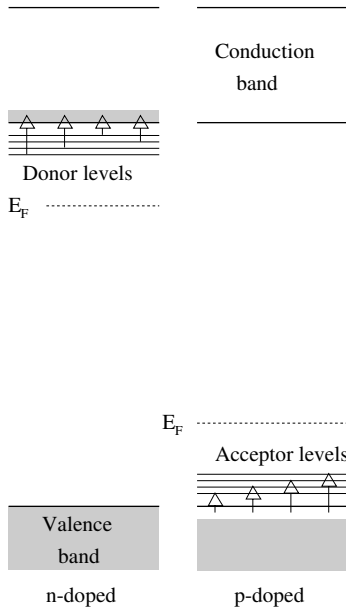
Fig. 14.19 Semiconductor energy levels produced by p- and n-doping. The arrows indicate the thermal excitation of electrons, as described in the text.
