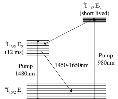
Fig. 16.20 \text{Er}^{3+} energy levels involved in erbium doped fibre amplification. Alternative pumping schemes are indicated.
