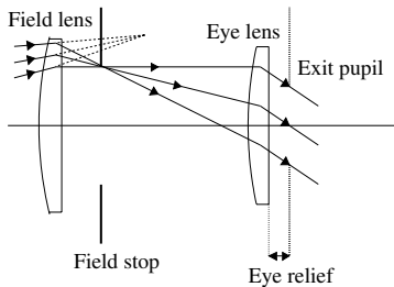
Fig. 4.4 Huygens' eyepiece.
