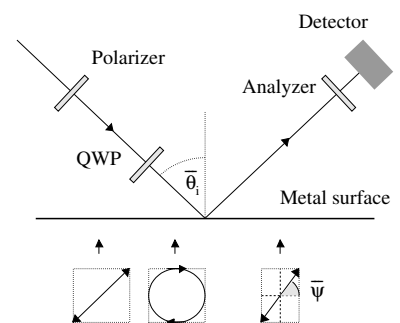
Fig. 11.7 Ellipsometer for determining the optical constants of metals. The successive polarization states are shown for a nulling measurement with light incident at the principal angle of incidence.
