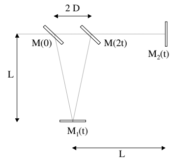
Fig. 5.13 Michelson–Morley experiment showing the position of the mirrors at the specified times in the conjectured aether.
