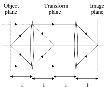
Fig. 7.24 4f architecture for coherent optical processing.
