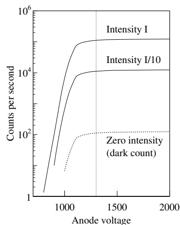
Fig. 15.27 Photomultiplier count rate versus applied voltage for beams of relative intensity I , 0.1I and 0 . The vertical line indicates the 'plateau' condition for valid count rates.
