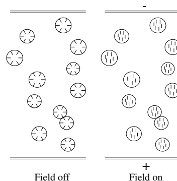
Fig. 10.28 Polymer dispersed liquid crystal. In the left hand panel the bubbles' refractive index is different from that of the polymer. In the right hand panel the refractive indices are the same for light incident normally.
