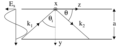
Fig. 9.22 A planar waveguide formed by plane parallel conducting surfaces. Wave vectors are drawn for the component plane waves making up the total wave that propagates within the gap. The electric field amplitude for one mode is drawn on the left.
