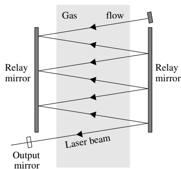
Fig. 14.8 Beam path and gas flow inside a CO 2 gas laser.
