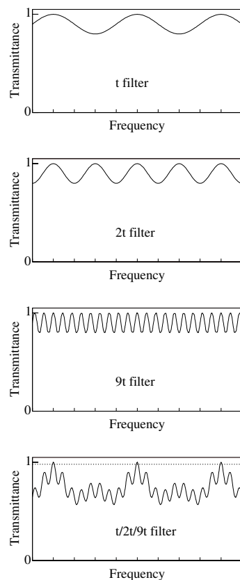
Fig. 14.36 Sketches of the transmittance through the layers of a birefringent filter. From the top downward in sequence: transmittance through plates of thickness t , 2t , 9t and through all three plates in series. The dotted line indicates notionally the transmittance at which the gain would be at its threshold value.
