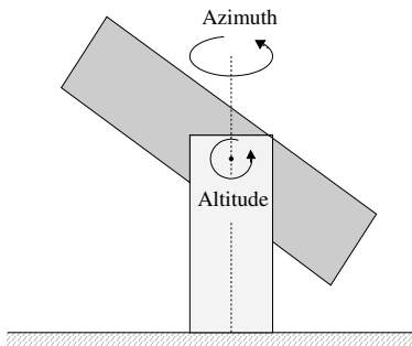
Fig. 8.4 Telescope in alt-az mounting.
