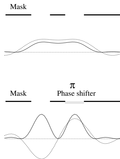
Fig. 6.29 Phase shift masking. The mask in the lower panel has a coating over one open region. The amplitudes and intensities at the wafer are shown with broken and full lines respectively.
