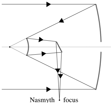
Fig. 8.7 Nasmyth focus along the altitude axis of a Cassegrain telescope in an alt-az mounting.
