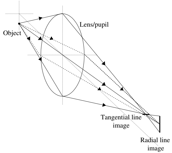
Fig. 3.25 Image formation with astigmatism. The solid lines are rays in the meridional plane containing the optical axis. The broken lines are sagittal rays forming a perpendicular line plane. These give tangential and radial line images respectively.
