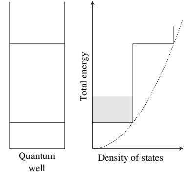
Fig. 14.28 Quantum well energy levels are shown in the left hand panel. In the right hand panel the density of states of the quantum well is shown as a full line and the density of states for an electron in bulk semiconductor by a broken line.
