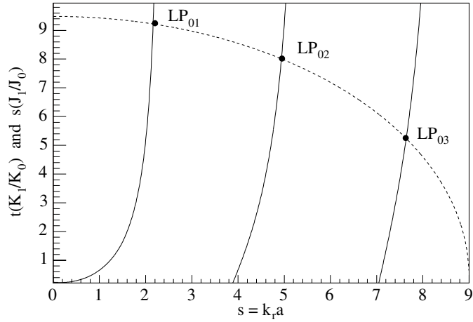
Fig. 16.2 Solutions to the characteristic equation for the propagation of LP_{0\ell} modes on optical fibre. The parameters are defined in the text. V is set to 9.0.
