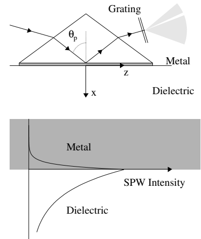
Fig. 11.14 The Kretschmann–Raether scheme for exciting surface plasma waves is shown in the upper panel. The lower panel shows the exponential decline in the intensity of the surface plasma wave with distance from the contact surface. The vertical scale is magnified in the lower panel.
