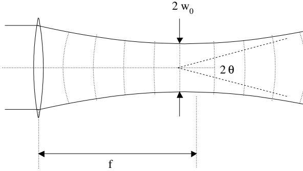
Fig. 6.32 Gaussian beam focused by an aberration-free lens. The curved dotted lines are wavefronts and the broken lines are asymptotic to the beam outline at a large distance along the axis.
