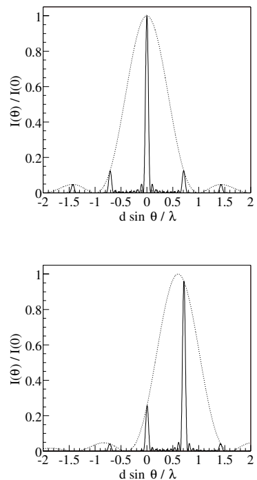
Fig. 6.16 The diffraction pattern seen with unblazed (upper panel) and blazed (lower panel) gratings.
