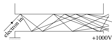
Fig. 15.28 Development of an electron cascade along an individual microchannel.
