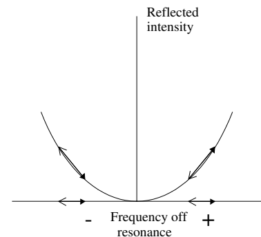
Fig. 8.23 The sign of the change in the reflected intensity from a Fabry–Perot cavity when the cavity length is increased reverses at resonance. This is equally true when changes are made instead in the laser frequency.
