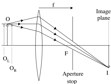
Fig. 4.16 A telecentric lens with the aperture stop located in the second focal plane.
