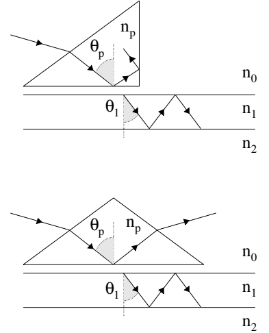
Fig. 9.24 Two prism coupler arrangements for launching light into a planar waveguide.
