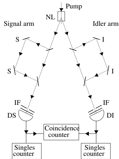
Fig. 18.11 Franson–Chiao interferometer used to observe two photon interference in which the idler and signal are not mixed.
