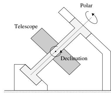
Fig. 8.5 Telescope in equatorial mounting.
