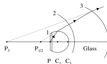
Fig. 4.8 Oil immersion objective showing conjugate points.
