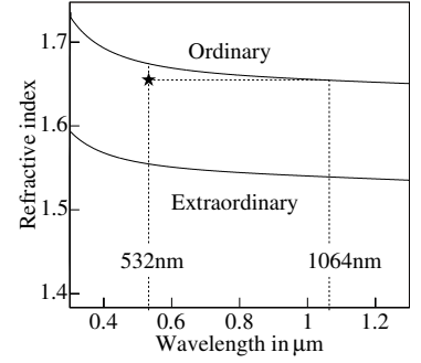
Fig. 14.42 Ordinary and extraordinary refractive indices for BBO. Type I phase matching is obtained at the position of the star for frequency doubling of a Nd:YAG laser beam.
