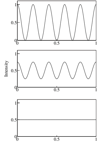
Fig. 7.5 Fringe visibility for two (top) fully coherent, (centre) partially coherent, and (bottom) incoherent sources.
