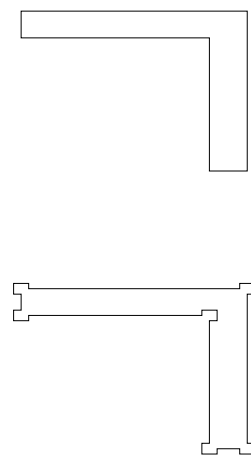
Fig. 6.30 A mask with optical proximity corrections is shown in the lower panel. This yields a satisfactory approximation to the shape shown above when projected onto the wafer.
