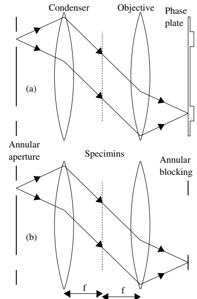
Fig. 7.14 The upper diagram shows phase contrast illumination, and the lower diagram shows dark field illumination.
