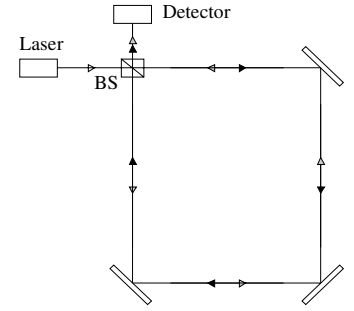
Fig. 5.22 Sagnac interferometer; passive ring gyro layout.
