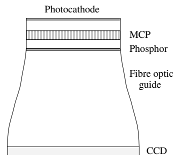
Fig. 15.29 Image intensifier based on a microchannel plate.
