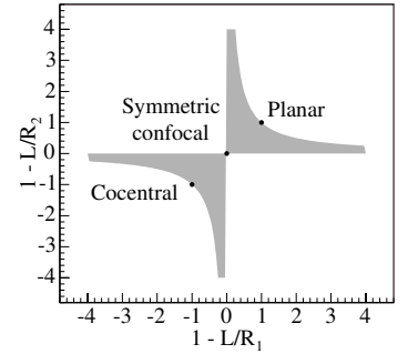
Fig. 6.34 Stability diagram for Fabry–Perot cavities.
