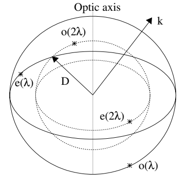
Fig. 14.43 Index ellipsoids for BBO at wavelengths 532 nm and 1064 nm. The orientation of the wave vector is that required to give type I phase matching when frequency doubling a Nd:YAG laser beam.
