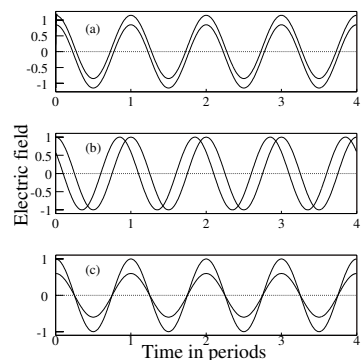
Fig. 18.2 The uncertainty spread in (a) a coherent wave; (b) the same wave after squeezing the amplitude uncertainty; (c) the same wave after squeezing the phase uncertainty. In each case the waves lie in the space between the two extremes shown.
