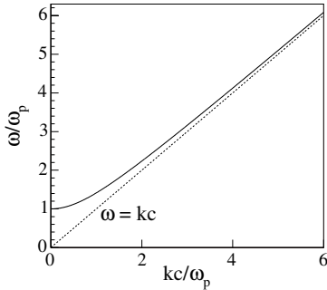
Fig. 11.11 Angular frequency variation with the wave number above the plasma frequency \omega_p . The dispersion relation for free space is also shown.
