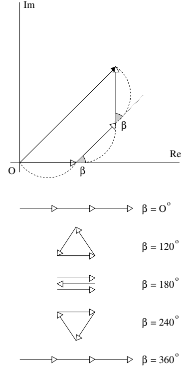
Fig. 6.7 Phasor diagrams for Fraunhofer diffraction at three equally spaced identical slits. The upper panel shows the slit phasors and their resultant. Below the alignments for intensity minima and maxima appear.
