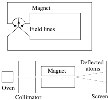
Fig. 13.12 The Stern–Gerlach experiment. The upper panel shows a section through the magnet perpendicular to the beam direction. The lower panel shows a vertical section containing the incident beam.
