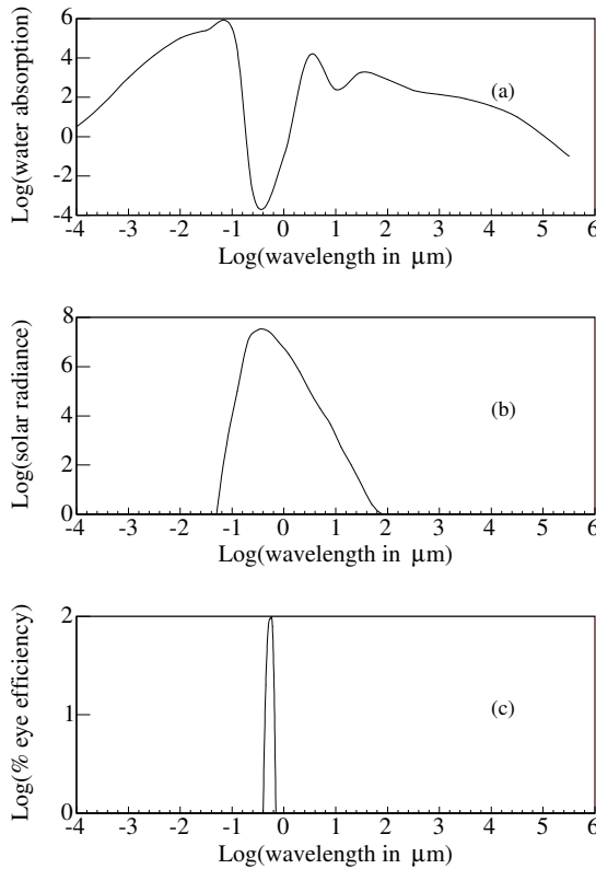
Fig. 1.17 Coincidences: (a) log of absorption coefficient for water in \text{cm}^{-1} ; (b) log of the Sun's spectral irradiance in \text{W m}^{-2} \mu\text{m}^{-1} (c) log of the relative spectral efficiency of the human eye.
