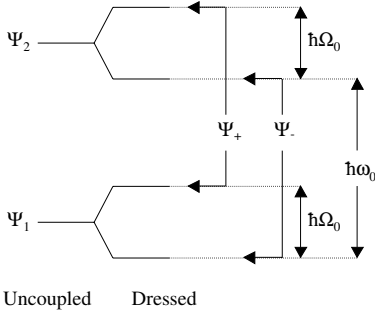
Fig. 17.4 Uncoupled and dressed atomic energy levels, for the case that the pump angular frequency equals the transition angular frequency \omega_0 .
