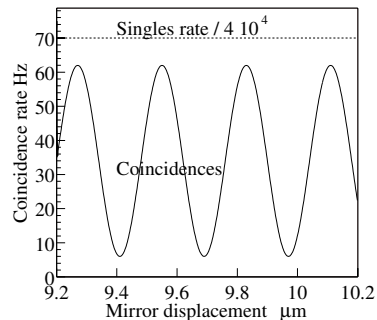
Fig. 18.12 Coincidence rate (solid line) and singles rate (broken line) in the measurement by P. G. Kwiat, A. M. Steinberg and R. Y. Chiao. The plots show smooth fits through the data appearing in Physical Review A47 2472 (1993). Courtesy Professor Chiao and the American Physical Society.
