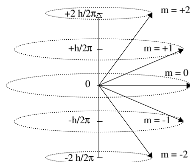
Fig. 13.11 Orientations of the angular momentum vector for the eigenstates with the orbital angular momentum quantum number equal to 2.
