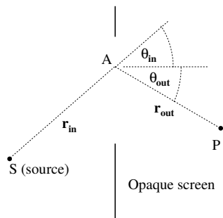
Fig. 6.1 Path lengths and angles used in Kirchhoff's analysis.
