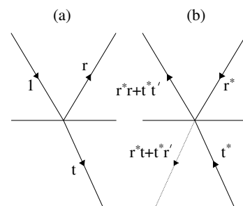
Fig. 5.17 Reflected and transmitted amplitudes: (a) for forward process and (b) for the time reversed process.
