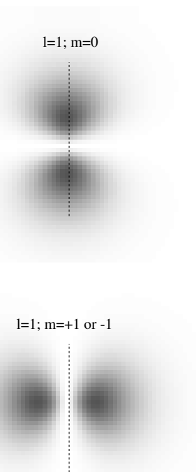
Fig. 13.10 Diametral sections through the probability distributions in the hydrogen atom for electrons in the 2p shell.
