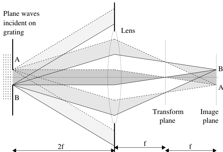
Fig. 7.12 Abbe's insight into image formation. The lower order diffractive beams from the grating AB are shown as shaded bands. A'B' is the grating image. Rays travelling from A to A' are drawn as broken lines; rays from B to B' as solid lines.
