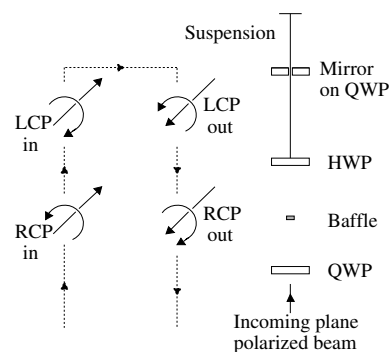
Fig. 13.16 Beth's experiment to observe the angular momentum of circularly polarized light. The right hand panel shows the optical equipment. The left hand panel indicates the state of polarization of the beam at each stage going in and out after reflection. Adapted from R. A. Beth, Physical Review Letters 50, 115 (1936), courtesy the American Physical Society.
