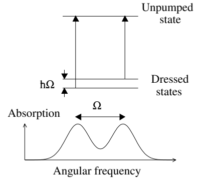
Fig. 17.7 Autler–Townes splitting of an absorption line: the transitions are shown above and the absorption spectrum below.
