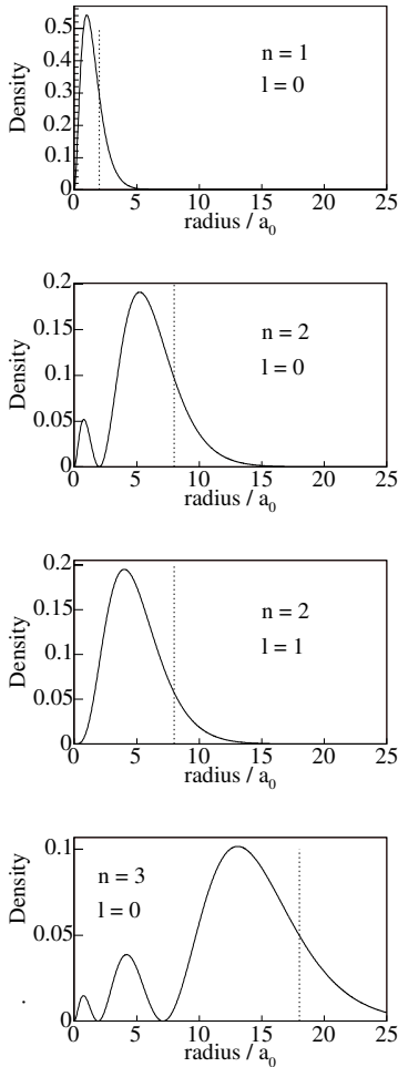
Fig. 13.9 Radial electron density distributions in the hydrogen atom for the lowest energy eigenstates. The dotted lines indicate where the kinetic energy changes sign.
