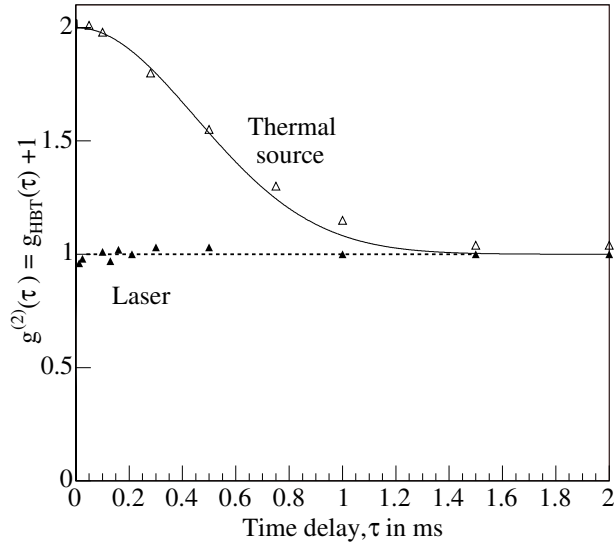
Fig. 18.1 The correlation between the arrival times of successive photons. Reprinted from ‘Time distribution of photons from coherent and Gaussian sources’ by Arecchi, Gatti and Sona in Physics Letters Vol. 20 pages 27–29, copyright 1966, with permission of Elsevier and Professor Arecchi.
