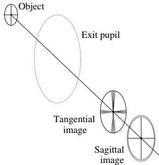
Fig. 3.26 Astigmatic image of a wheel-shaped object centred on the optical axis. At the tangential focus radial lines blurred and at the sagittal focus the tangential lines are blurred.
