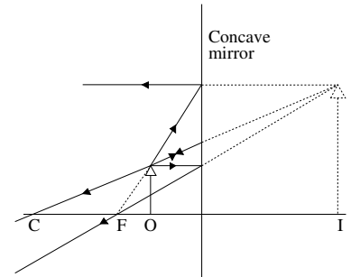
Fig. 3.5 Ray tracing for an object O in front of a concave mirror with centre of curvature C and focal point F. The image is formed at I. Rays are solid lines, construction lines are broken.
