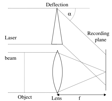
Fig. 7.25 Setup for producing a VanderLugt filter.
