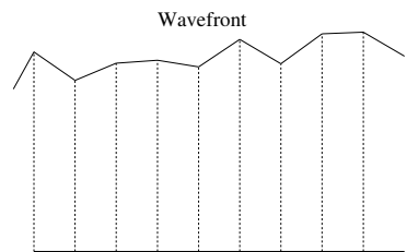
Fig. 8.11 Wavefront segments reconstructed by the Shack–Hartman wavefront sensor.
