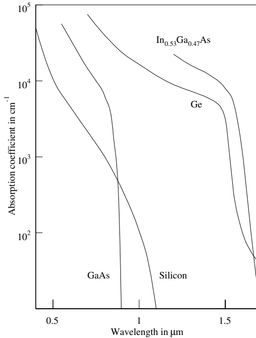
Fig. 15.1 Absorption coefficients of several semiconductors: adapted from J. M. Senior Optical Fibre Communications: Principles and Practice , second edition 1992, published by Pearson/Prentice-Hall International, Englewood Cliffs, New Jersey. Courtesy Dr Senior and Pearson Publishing.
