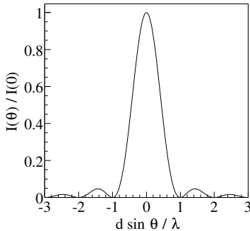
Fig. 6.4 Intensity distribution for Fraunhofer diffraction at a finite width slit.
