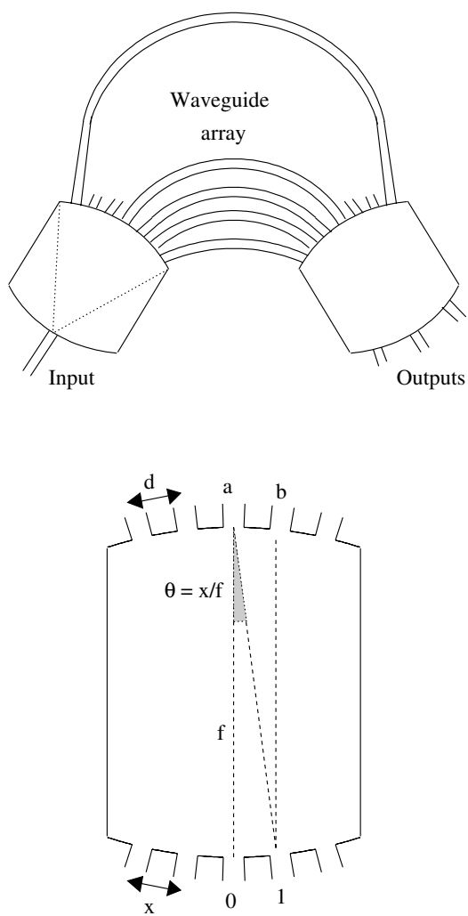
Fig. 16.26 Array waveguide grating. The upper panel shows both slabs and the waveguide array. The lower panel shows details of the second slab. The ports labelled a and b are the input ports, those labelled 0 and 1 are output ports.
