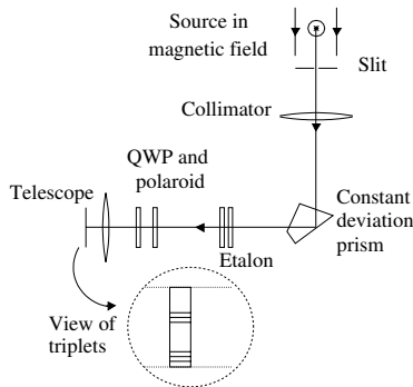
Fig. 13.17 Apparatus for viewing the polarization states of Zeeman split lines.
