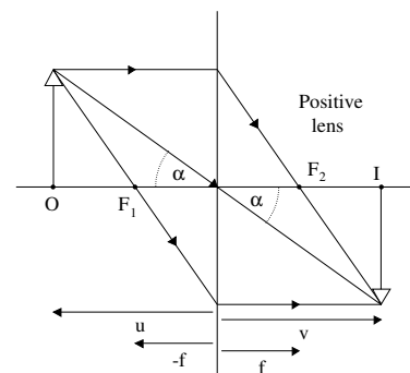
Fig. 3.12 Ray tracing through a positive lens. The object at O produces a real image at I.
