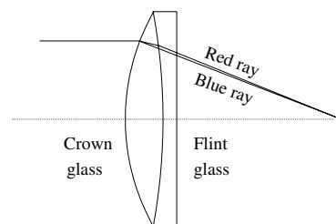
Fig. 3.34 Achromat doublet lens.
