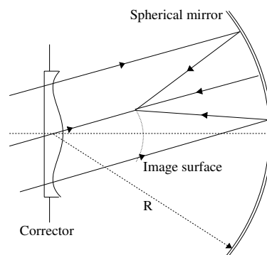
Fig. 8.8 Schmidt camera.
