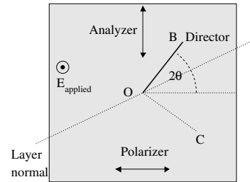
Fig. 10.30 Surface stabilized ferroelectric liquid crystal cell, seen face on. The alignments of the directors are shown for alternative signs of the applied electric field across the cell.
