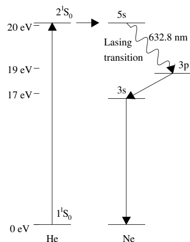
Fig. 14.3 He:Ne electron energy levels relevant to lasing at 632.8 nm.
