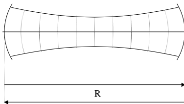
Fig. 6.31 Gaussian beam confined in a symmetric confocal Fabry-Perot cavity. The curved broken lines are wavefronts.
