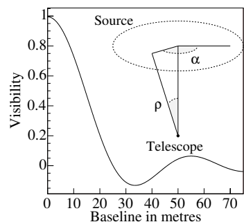
Fig. 8.18 Visibility versus baseline for a 20 mas source observed at a wavelength of 2.2 \mu\text{m} .
