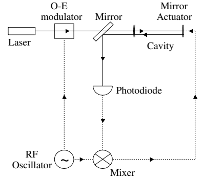
Fig. 8.24 Pound–Drever stabilization scheme. This locks the Fabry–Perot cavity length to an integral multiple of half wavelengths of a laser. The solid lines show the light paths while the broken lines carry electronic signals.
