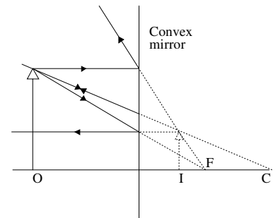
Fig. 3.6 Ray tracing for an object O in front of a convex mirror centre of curvature C and focal point F. The image is formed at I. Rays are solid lines, construction lines are broken.
