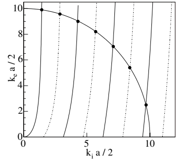
Fig. 13.3 Graphical method for obtaining solutions of Schrodinger's equation for the square well potential of depth V_0 and width a . k_i is the wavenumber within the well, and k_e that outside it. The curves are discussed in the text.
