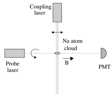
Fig. 17.9 Sketch of apparatus used by Hau and colleagues to observe electromagnetically induced transparency in a cloud of ultracold sodium atoms.
