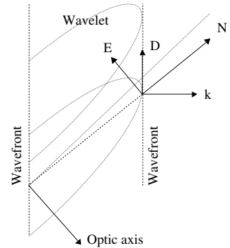
Fig. 10.8 Huygens' construction for a plane wave travelling in a negative uniaxial crystal.
