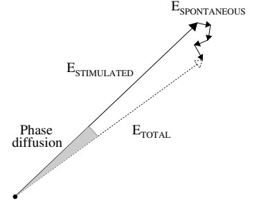
Fig. 14.26 Diffusion of the laser phase due to spontaneous emission.
