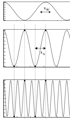
Fig. 7.10 In the upper panel the scan length, x_w , is much shorter than the wavelength. In the lower panels aliasing is shown between sine waves of wavelength 2x_s and 2x_s/3 for a sampling interval x_s . Samplings are indicated by dots.
