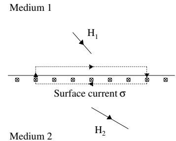
Fig. 9.3 Integration loop straddling an interface between media.
