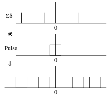
Fig. 7.2 The figure shows the convolution of a sum of delta functions with a square pulse. The resultant is a set of square pulses centred on the delta function locations.
