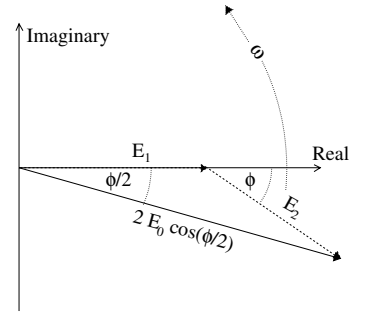
Fig. 5.5 Phasor diagram for Young's two slit experiment.
