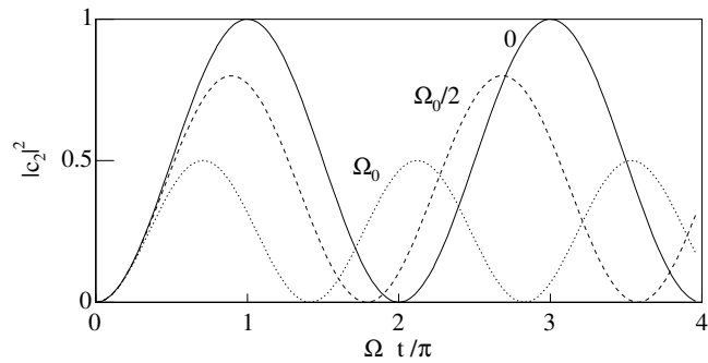
Fig. 17.2 Time dependence of the upper state population for different offsets of the pump angular frequency from the transition angular frequency. The offsets are \Delta\omega = 0 , \Omega_0/2 and \Omega_0 .
