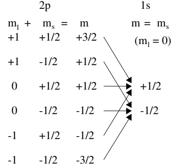
Fig. 17.1 Allowed transitions in hydrogen between the magnetic substates of the 2p and 1s states.
