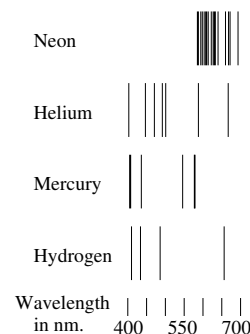
Fig. 2.11 Spectral lines observed with lamps containing gases of various elements at low pressure.
