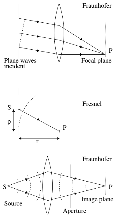
Fig. 6.21 Examples of Fraunhofer diffraction (upper and lower panels), and Fresnel diffraction (centre panel).
