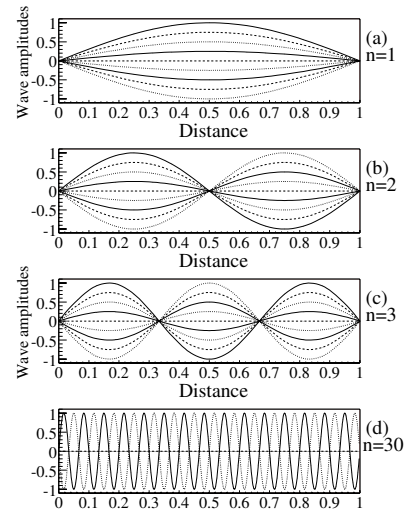
Fig. 5.27 Standing wave patterns for (a) the n = 1 mode, (b) the n = 2 mode, (c) the n = 3 mode, (d) the n = 30 mode. In (a), (b), and (c) the waves are shown at intervals of \tau/16 , and at intervals of \tau/2 in (d).
