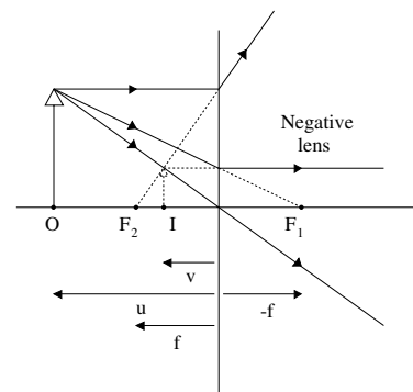
Fig. 3.13 Ray tracing through a negative lens. The object at O produces a virtual image at I.
