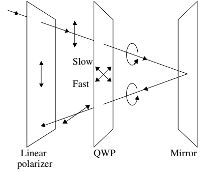
Fig. 10.10 Linear polarizer and quarter-wave plate used to suppress the reflections of ambient light from a screen. The screen is treated as a mirror. The polarization state of the light at each step is shown.
