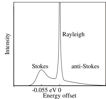
Fig. 14.48 The spectrum of light after traversing a long span of optical fibre.
