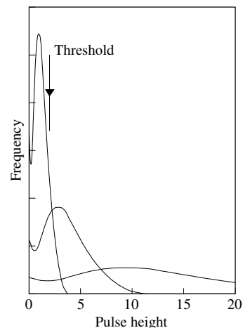
Fig. 15.26 Photomultiplier pulse height distributions for three different anode voltages. The number of pulses is the same for all three plots.
