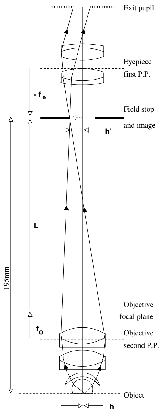
Fig. 4.9 Microscope construction showing the ray cone collected from an off-axis object point.
