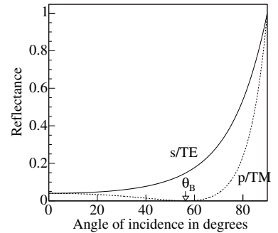
Fig. 9.14 Reflectance for both s- and p-polarization when light is incident in air on a plane glass surface. The glass has refractive index 1.5.
