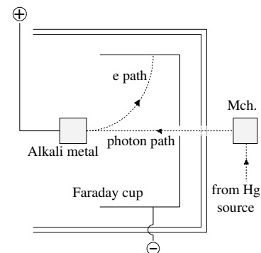
Fig. 12.3 Millikan's apparatus to study the photoelectric effect. Mch is a monochromator. The light passes through a window in the container.
