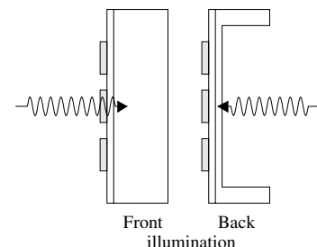
Fig. 15.20 Comparison of front illumination of a standard CCD and back illumination of a thinned CCD.
