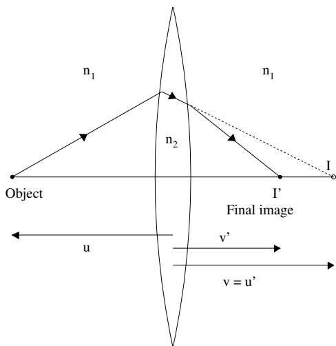
Fig. 3.8 Formation of an image of an object on the optical axis of a thin lens. The intermediate image produced by refraction at the first lens' surface is I . This is imaged by refraction at the second surface at I' .
