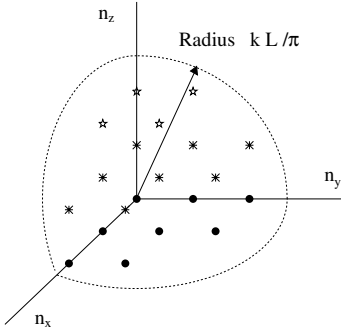
Fig. 9.21 The space displaying the electromagnetic modes in a reference volume. The labelling is explained in the text.
