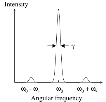
Fig. 17.13 Absorption spectrum around the 282 nm transition for Doppler cooled mercury ions. Only the stronger, first sidebands are shown.
