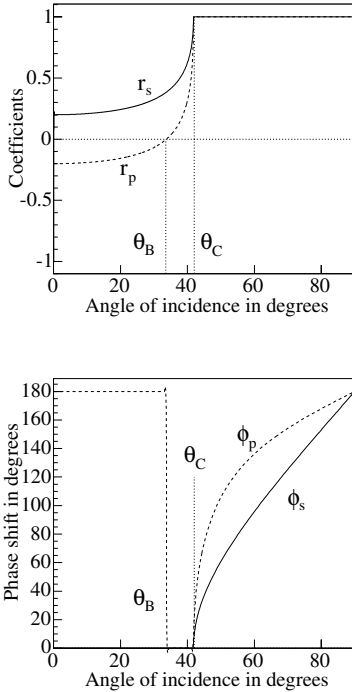
Fig. 9.15 The variation of the reflection amplitude coefficient with the angle of incidence on a plane interface between two dielectrics for both s- and p-polarization in the case that the light is incident in the optically denser dielectric. The refractive indices are chosen to be 1.5 and 1.0. In the upper panel the magnitudes of the coefficients are shown and in the lower panel their phases relative to the incident radiation. \theta_B is Brewster's angle and \theta_c is the critical angle.
