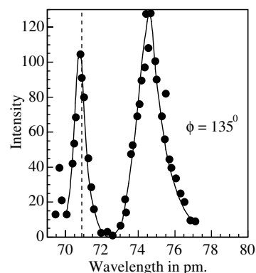
Fig. 12.7 Wavelength distribution of X-rays scattered from graphite. The vertical line indicates the wavelength of the direct beam (the K_\alpha line of Molybdenum.). Taken from A. H. Compton, Physical Review 22, 411 (1923), by courtesy of the American Physical Society.
