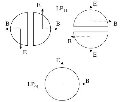
Fig. 16.4 Sketches of the cross-sections and field orientations in the LP_{01} and LP_{11} modes. In each case drawn there are orthogonal modes which have the electric and magnetic field directions exchanged.
