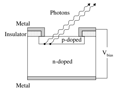
Fig. 14.21 A cross-section through a light emitting diode. The outer dimensions in this plane are a few microns.
