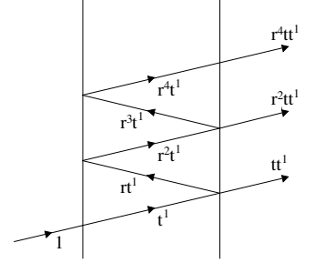
Fig. 5.30 Successive contributions to the wave amplitude transmitted by a Fabry-Perot etalon.
